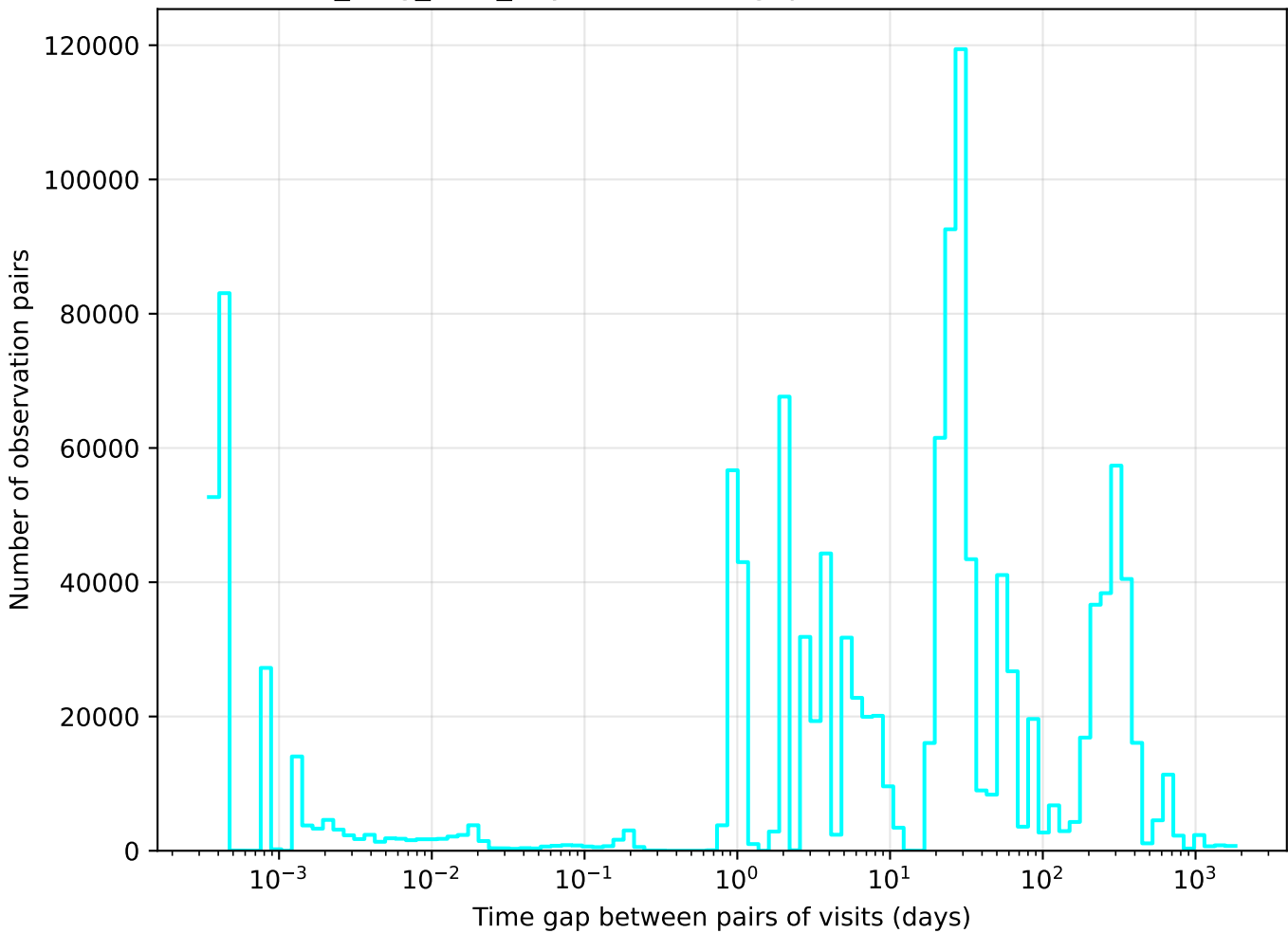
all_long_v3.4_10yrs u band: Tgaps observationStartMJD
