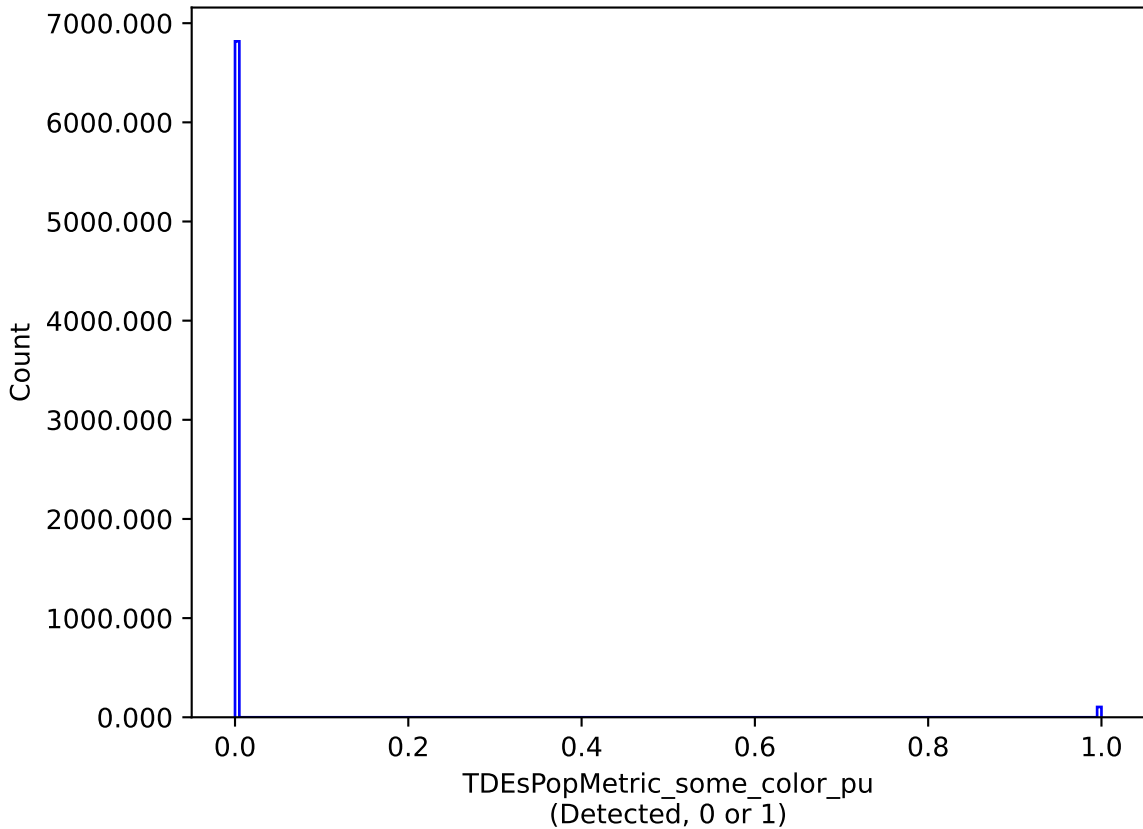
all_long_v3.4_10yrs : TDEsPopMetric_some_color_pu
