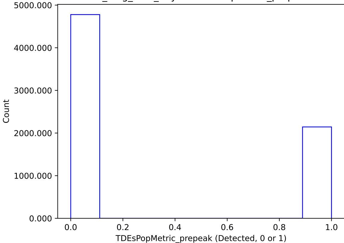
all_long_v3.4_10yrs : TDEsPopMetric_prepeak
