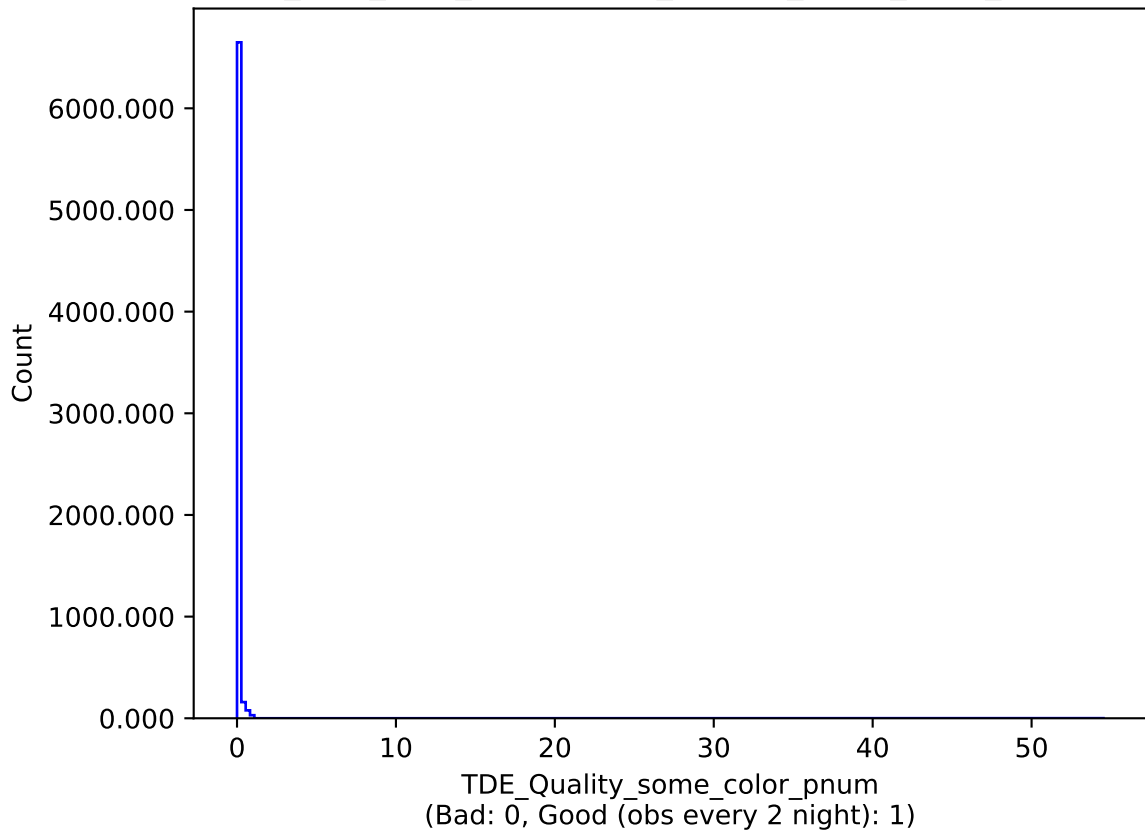
all_long_v3.4_10yrs : TDE_Quality_some_color_pnum
