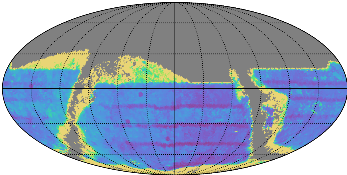
all_long_v3.4_10yrs : TDC_accuracy
