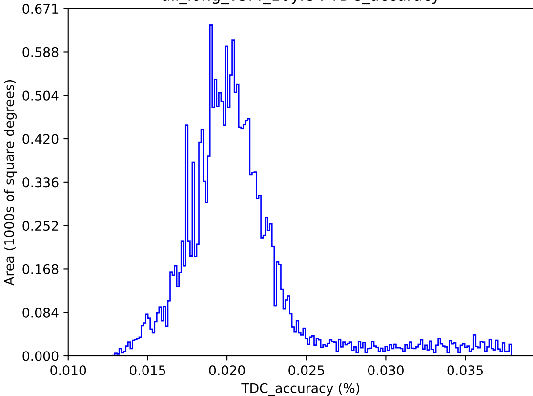
all_long_v3.4_10yrs : TDC_accuracy
