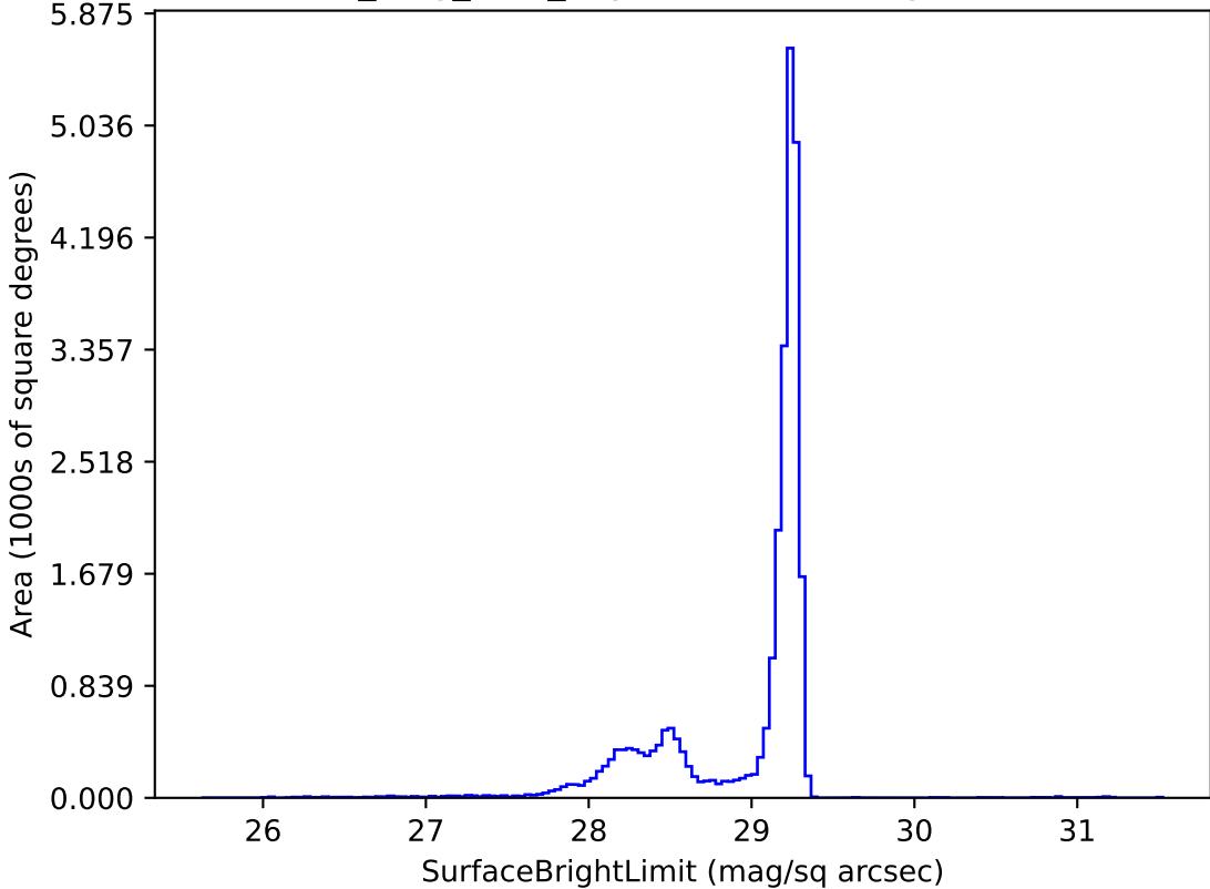
all_long_v3.4_10yrs z: SurfaceBrightLimit
