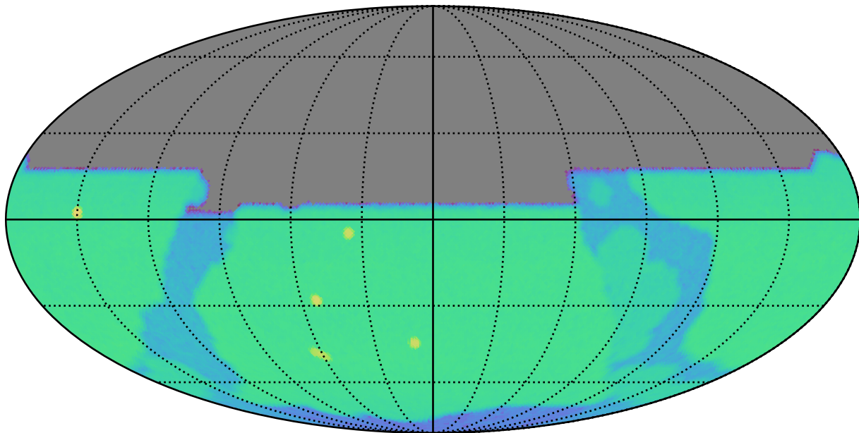
all_long_v3.4_10yrs y: SurfaceBrightLimit
