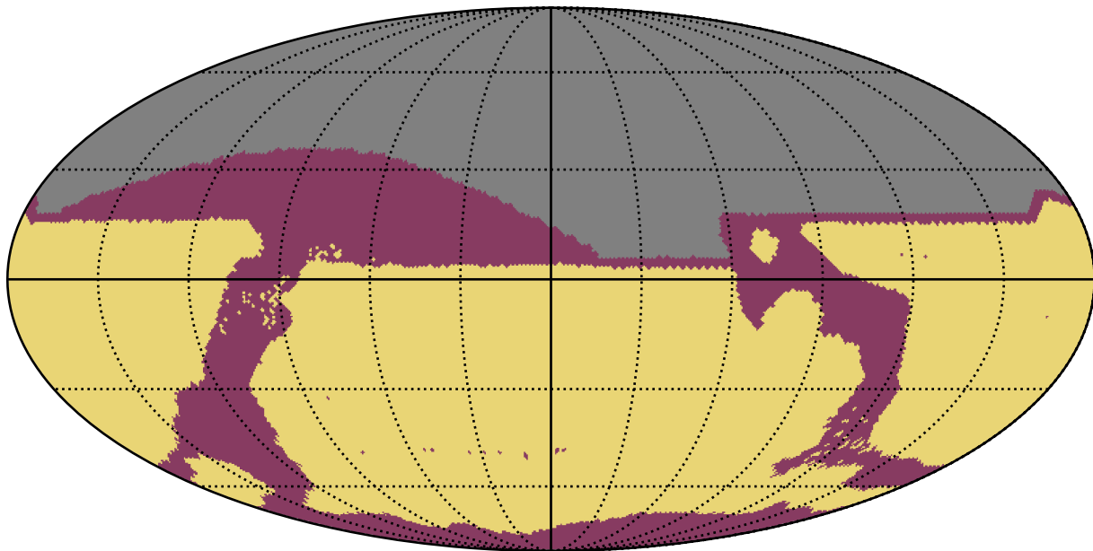
all_long_v3.4_10yrs : RapidRevisits
