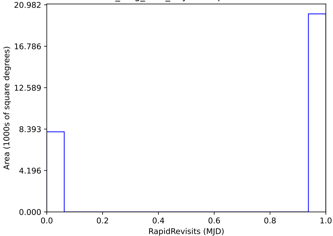
all_long_v3.4_10yrs : RapidRevisits
