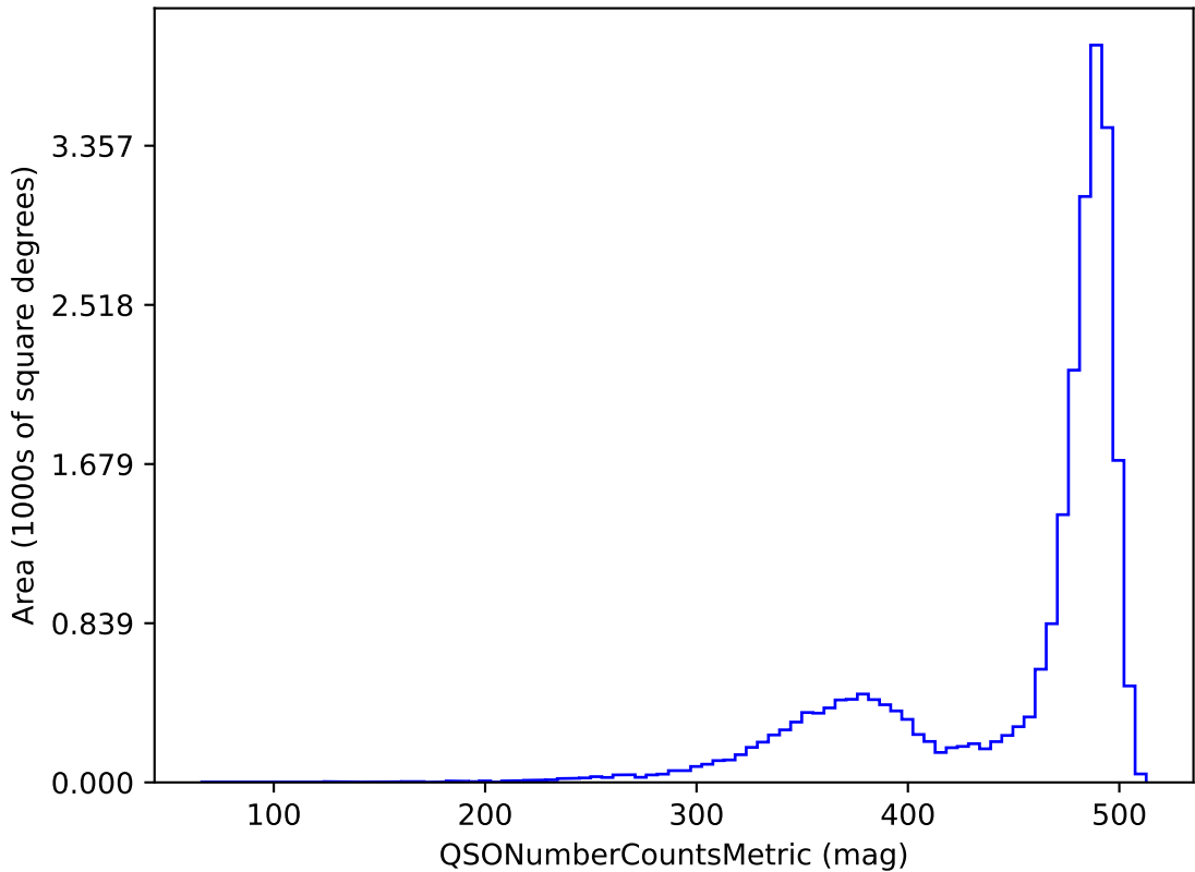
all_long_v3.4_10yrs z band and non-DD: QSONumberCountsMetric
