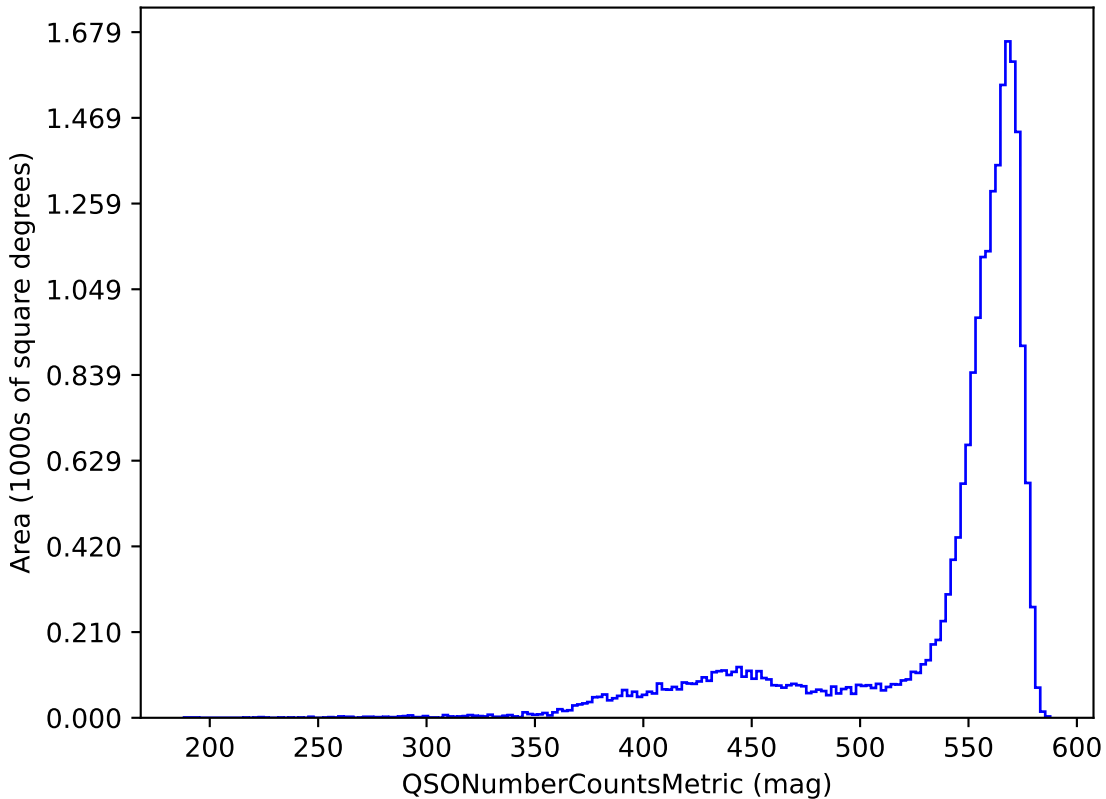
all_long_v3.4_10yrs y band and non-DD: QSONumberCountsMetric
