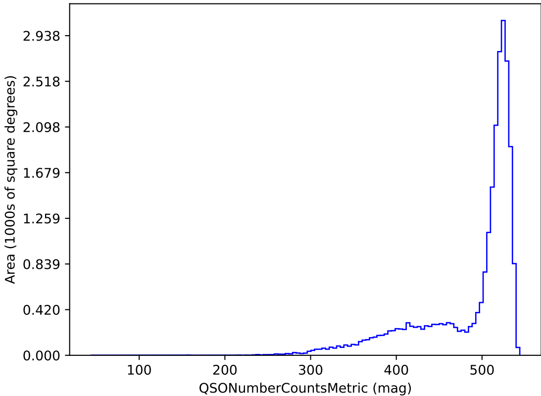
all_long_v3.4_10yrs r band and non-DD: QSONumberCountsMetric
