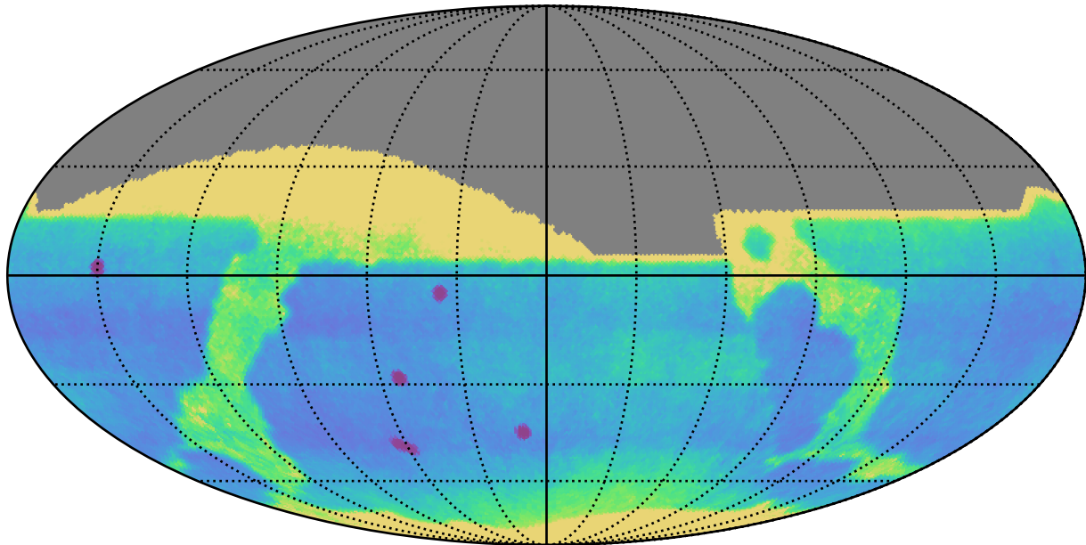
all_long_v3.4_10yrs : Proper Motion Uncert @ 24.0
