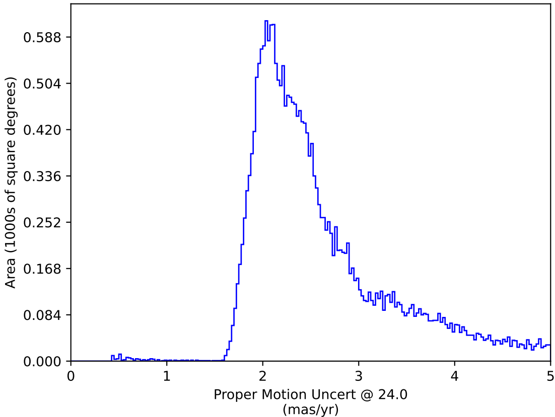
all_long_v3.4_10yrs : Proper Motion Uncert @ 24.0
