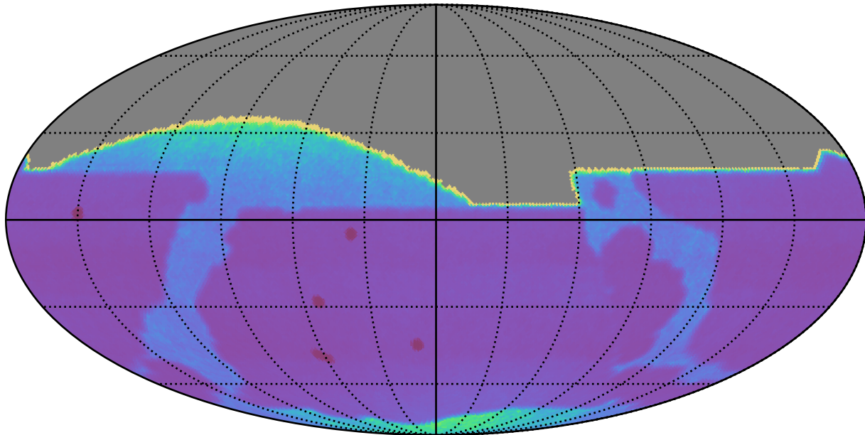
all_long_v3.4_10yrs : Proper Motion Uncert @ 20.5
