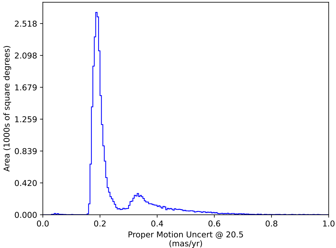
all_long_v3.4_10yrs : Proper Motion Uncert @ 20.5
