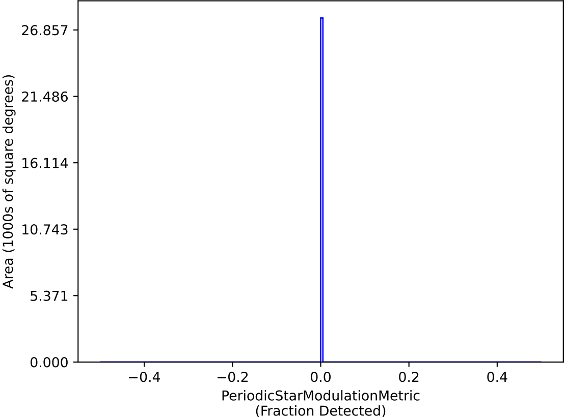
all_long_v3.4_10yrs dm 19 interval 15 RRC Year 1-2: PeriodicStarModulationMetric
