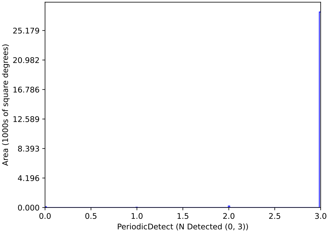
all_long_v3.4_10yrs P_2.0_Mag_21_Amp_0.05-0.1-1: PeriodicDetect
