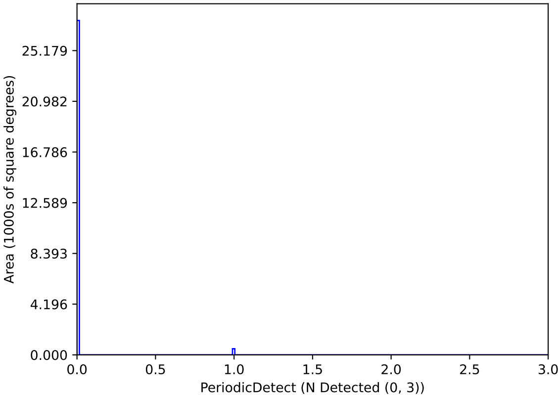
all_long_v3.4_10yrs P_1.0_Mag_24_Amp_0.05-0.1-1: PeriodicDetect
