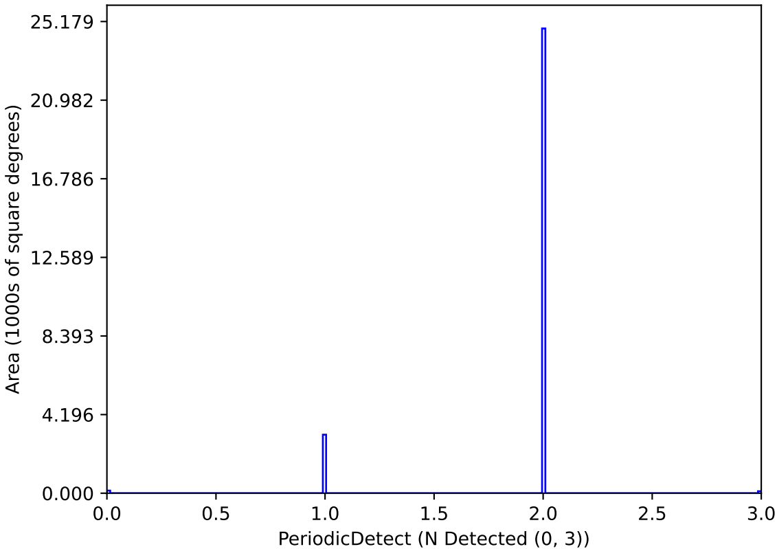
all_long_v3.4_10yrs P_1.0_Mag_21_Amp_0.05-0.1-1: PeriodicDetect
