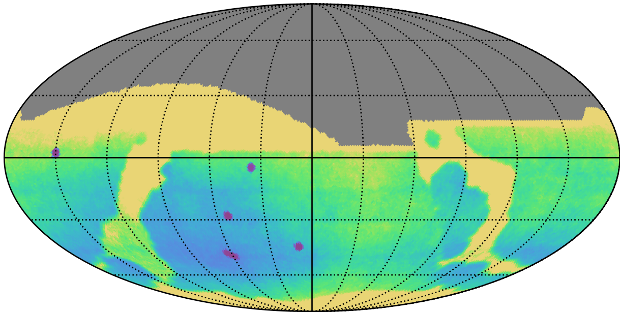
all_long_v3.4_10yrs : Parallax Uncert @ 24.0
