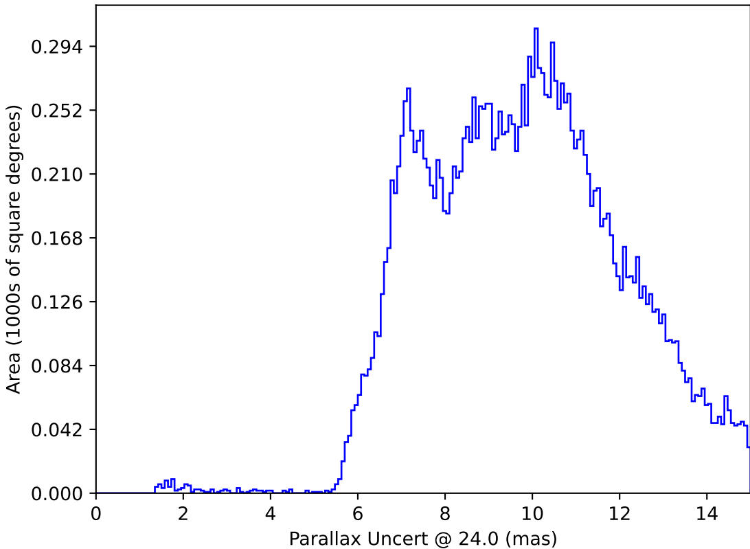
all_long_v3.4_10yrs : Parallax Uncert @ 24.0
