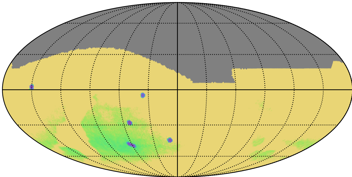
all_long_v3.4_10yrs : Parallax Uncert @ 22.4
