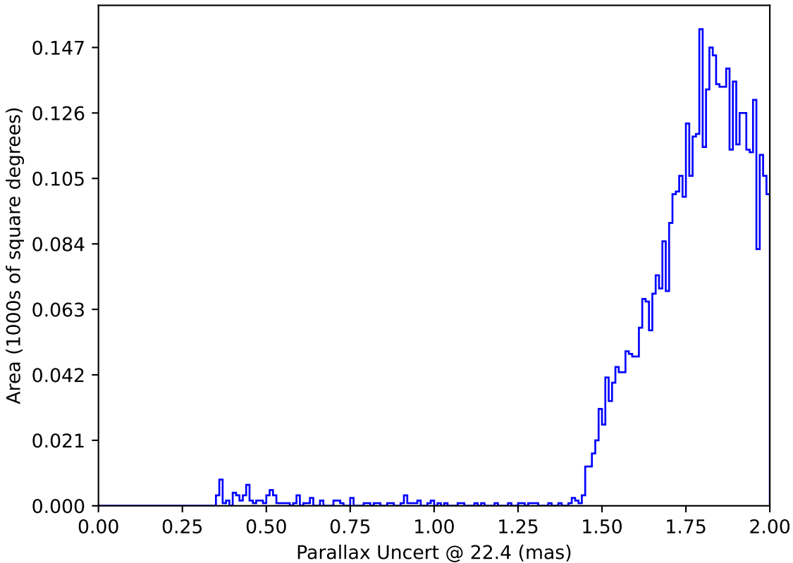
all_long_v3.4_10yrs : Parallax Uncert @ 22.4
