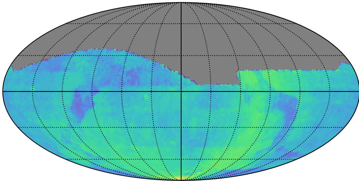
all_long_v3.4_10yrs : Parallax Coverage @ 24.0
