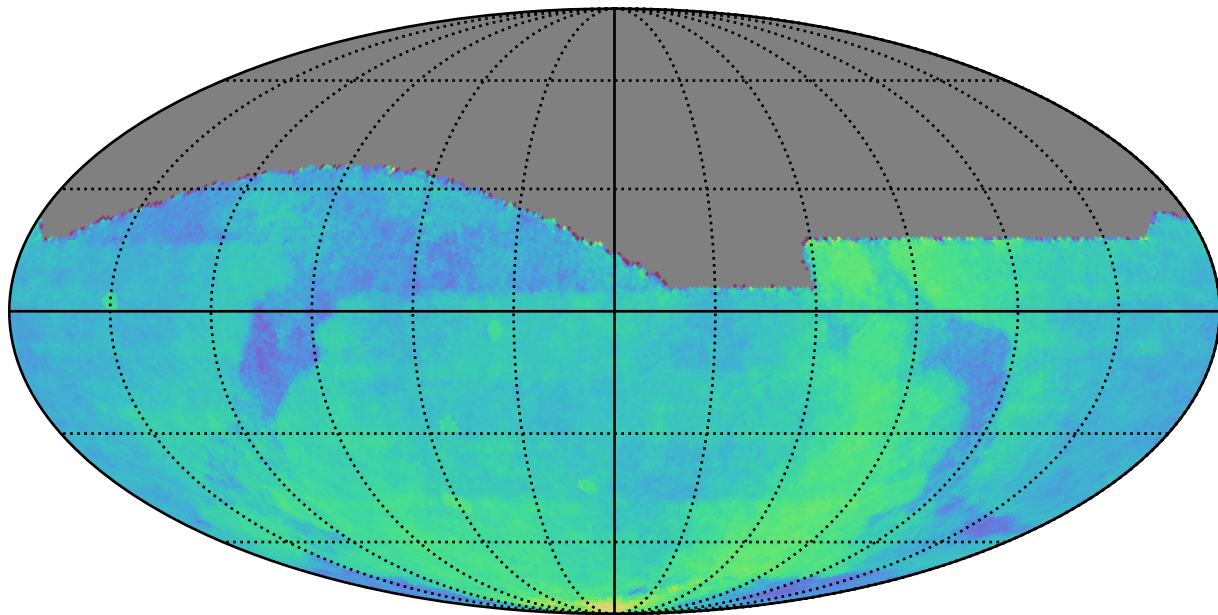
all_long_v3.4_10yrs : Parallax Coverage @ 22.4
