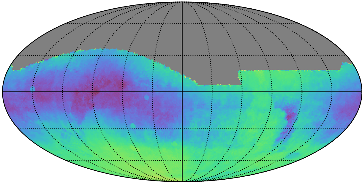
all_long_v3.4_10yrs : Parallax-DCR degeneracy @ 24.0
