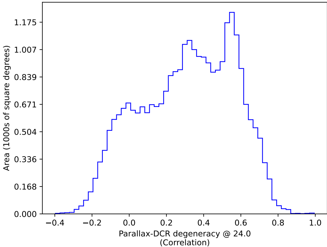
all_long_v3.4_10yrs : Parallax-DCR degeneracy @ 24.0
