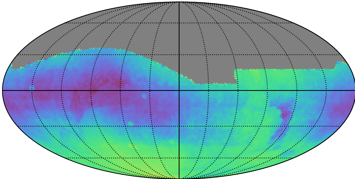
all_long_v3.4_10yrs : Parallax-DCR degeneracy @ 22.4
