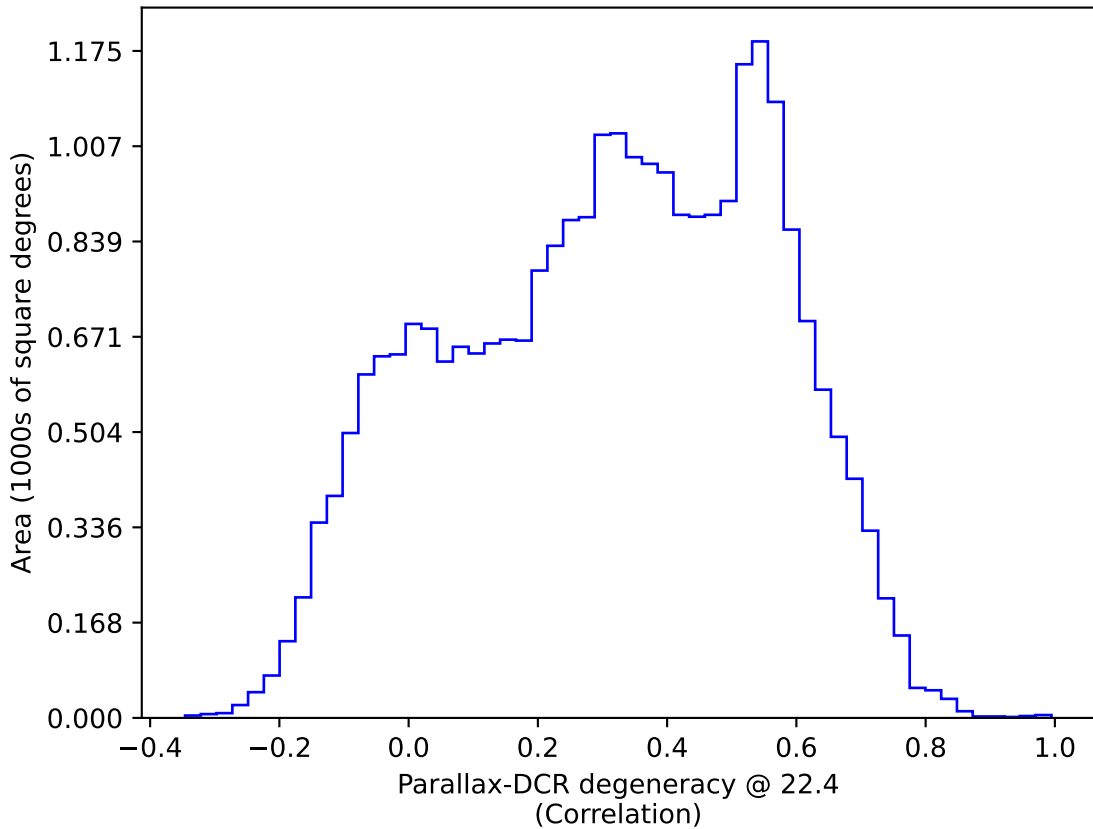
all_long_v3.4_10yrs : Parallax-DCR degeneracy @ 22.4
