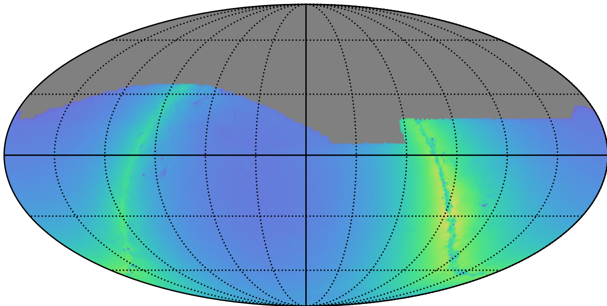
all_long_v3.4_10yrs r: Nstars_no_crowding
