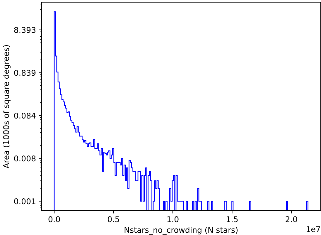
all_long_v3.4_10yrs r: Nstars_no_crowding
