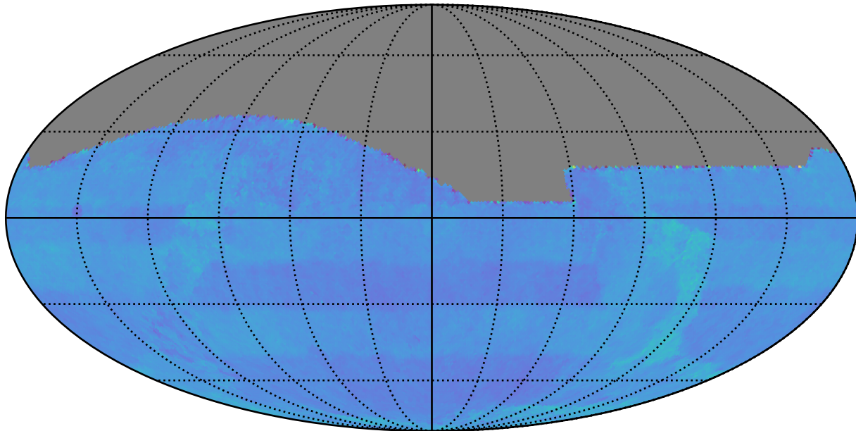
all_long_v3.4_10yrs : Normalized Proper Motion Uncert @ 24.0
