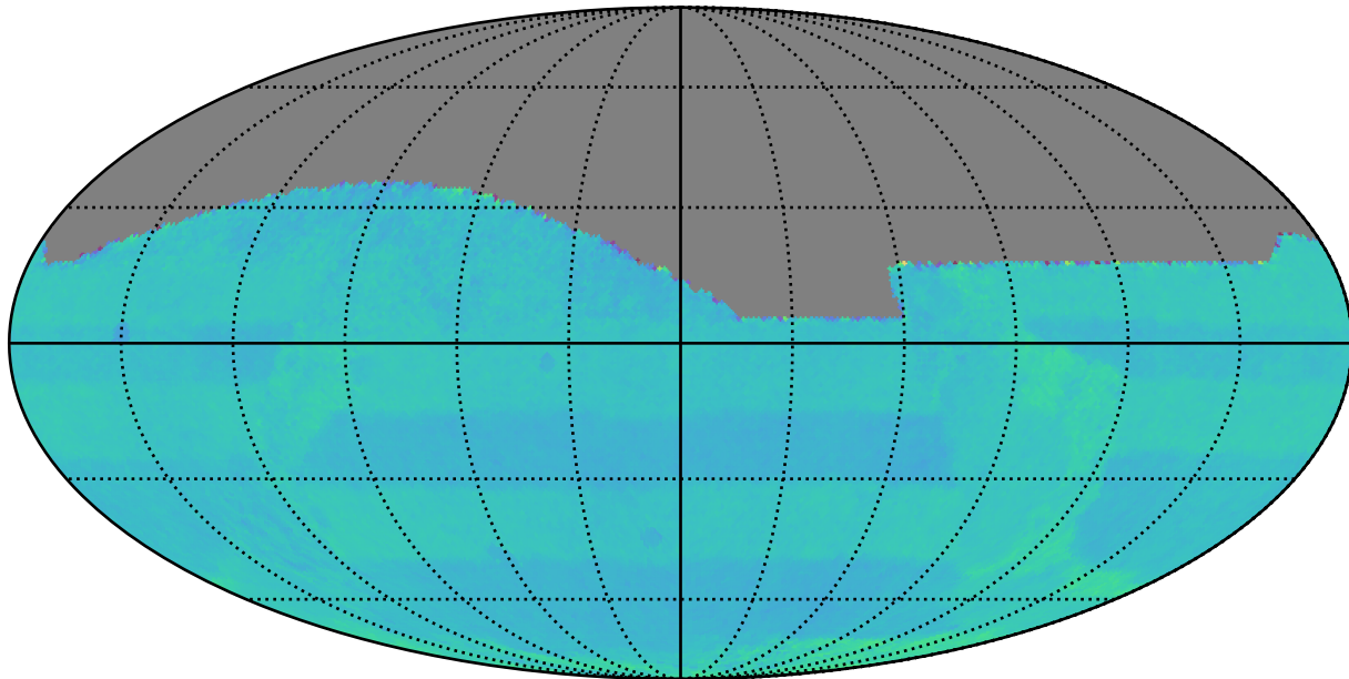
all_long_v3.4_10yrs : Normalized Proper Motion Uncert @ 20.5
