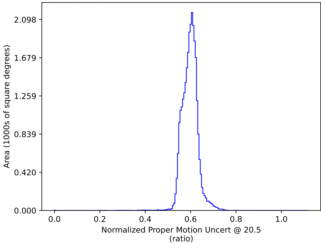
all_long_v3.4_10yrs : Normalized Proper Motion Uncert @ 20.5
