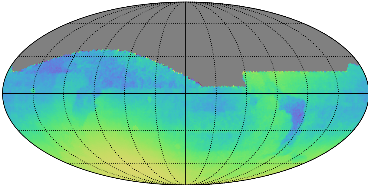
all_long_v3.4_10yrs : Normalized Parallax Uncert @ 24.0
