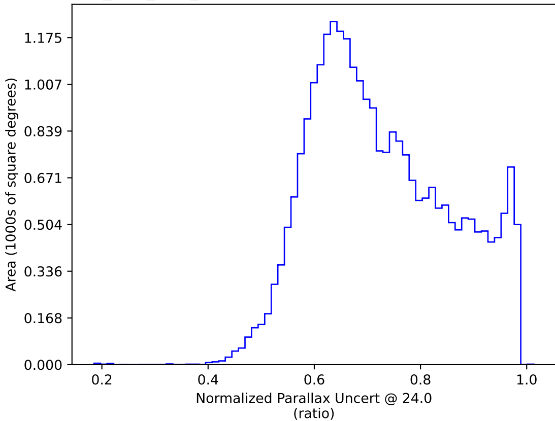
all_long_v3.4_10yrs : Normalized Parallax Uncert @ 24.0
