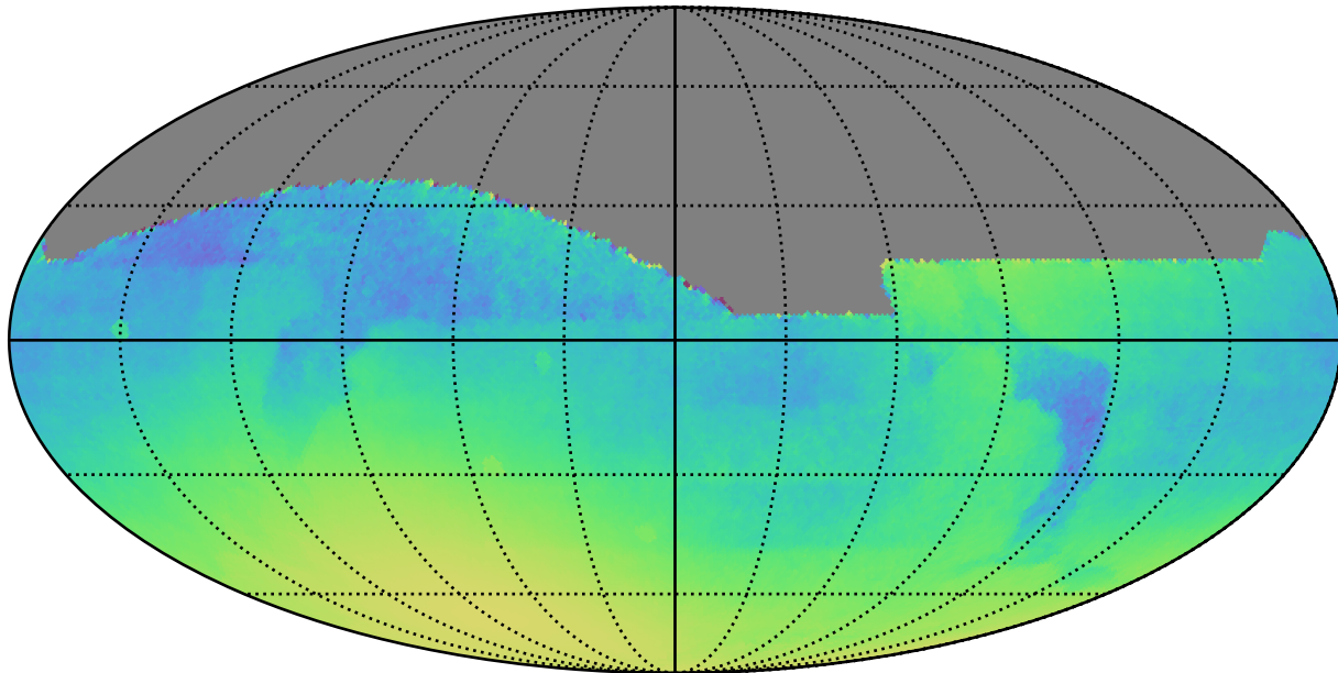
all_long_v3.4_10yrs : Normalized Parallax Uncert @ 22.4
