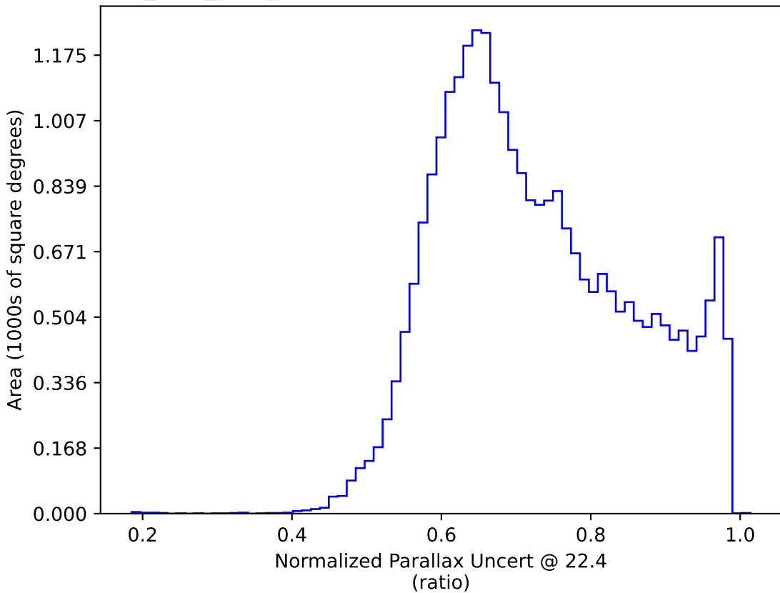
all_long_v3.4_10yrs : Normalized Parallax Uncert @ 22.4
