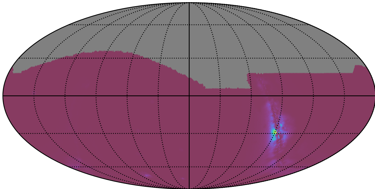
all_long_v3.4_10yrs : NlcPoints
