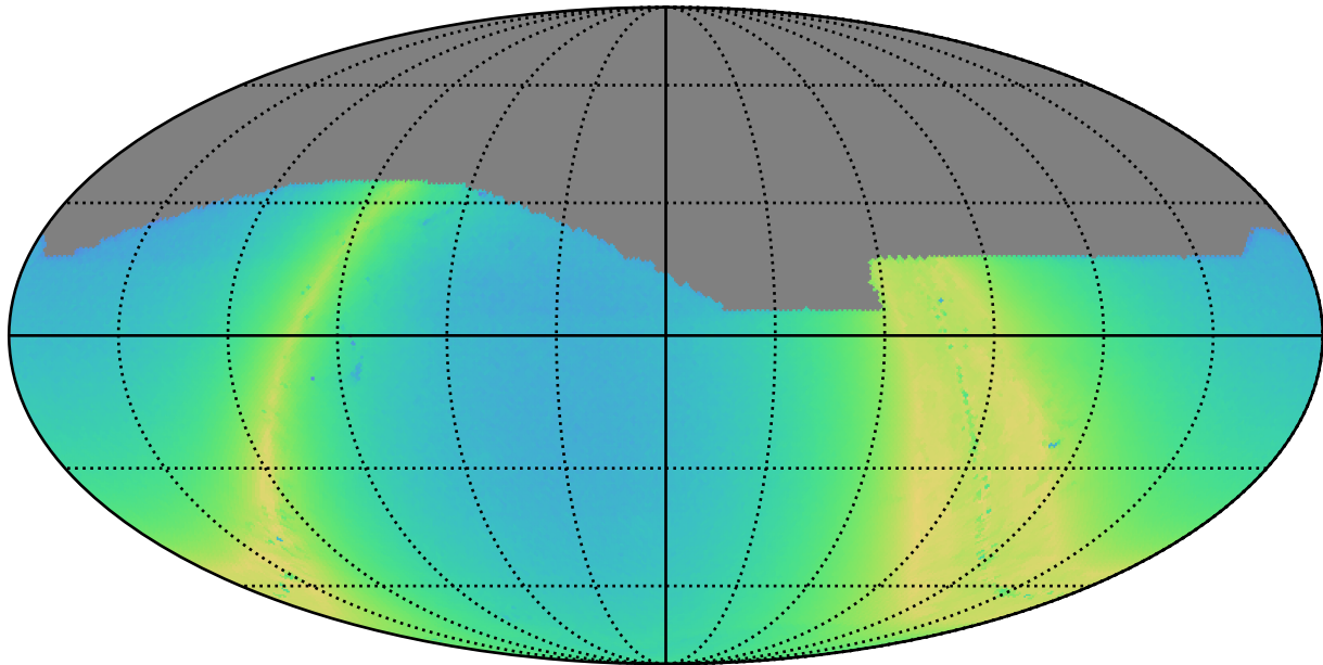
all_long_v3.4_10yrs z: N stars to Precision 0.20
