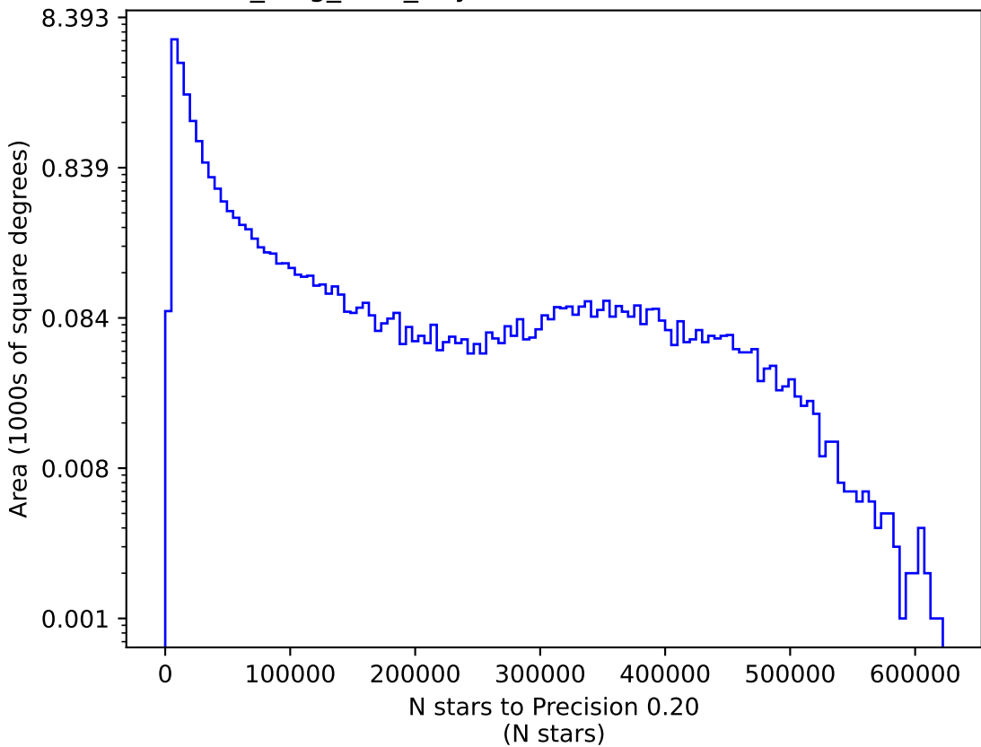
all_long_v3.4_10yrs z: N stars to Precision 0.20
