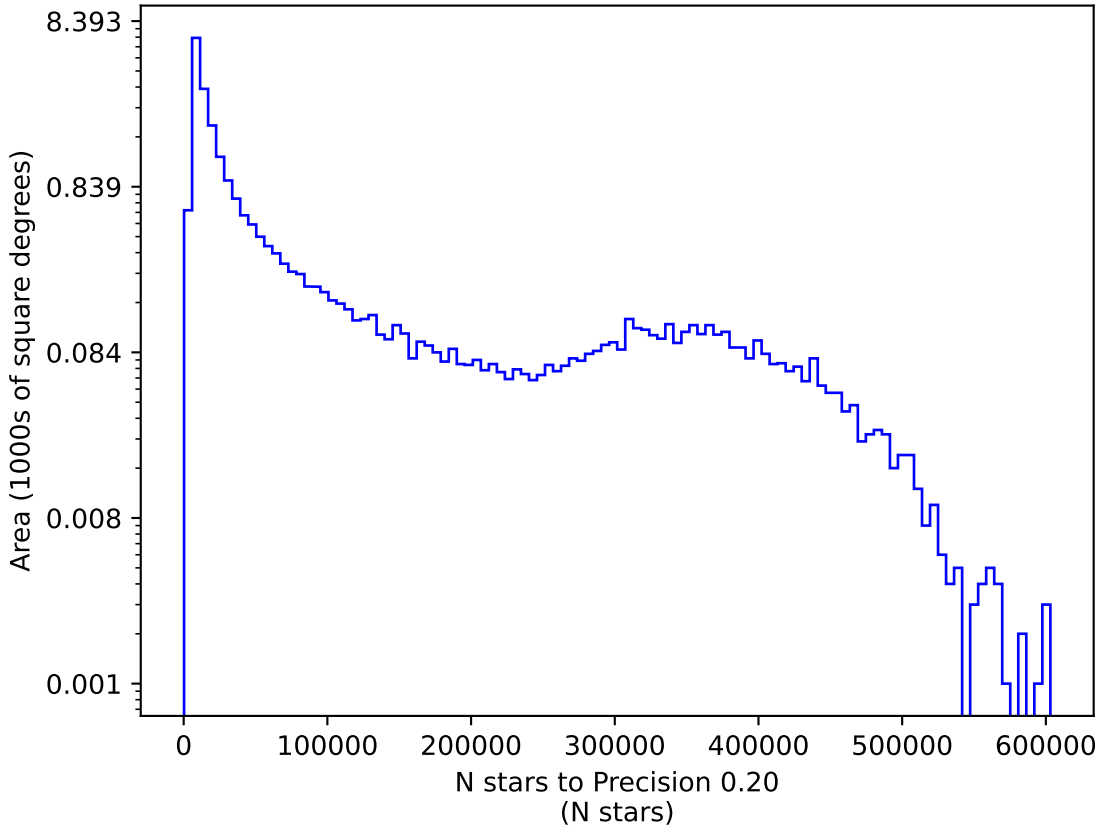
all_long_v3.4_10yrs y: N stars to Precision 0.20
