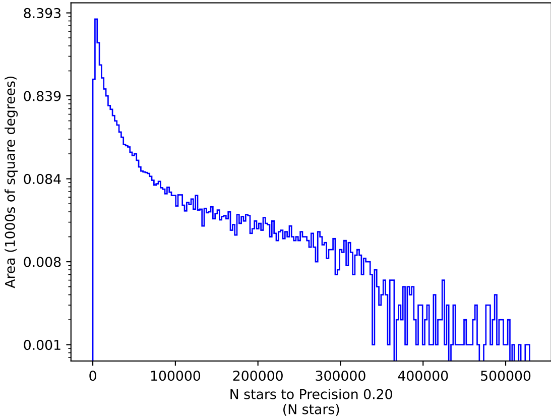
all_long_v3.4_10yrs u: N stars to Precision 0.20
