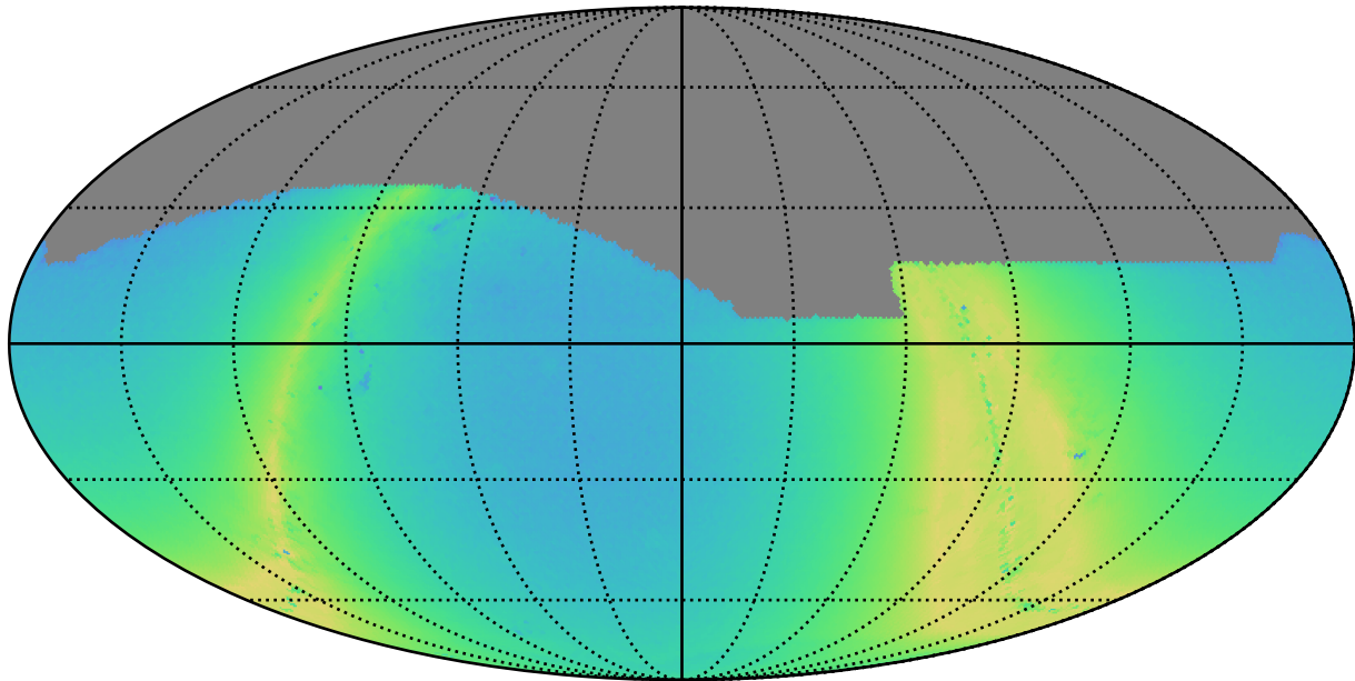
all_long_v3.4_10yrs r: N stars to Precision 0.20
