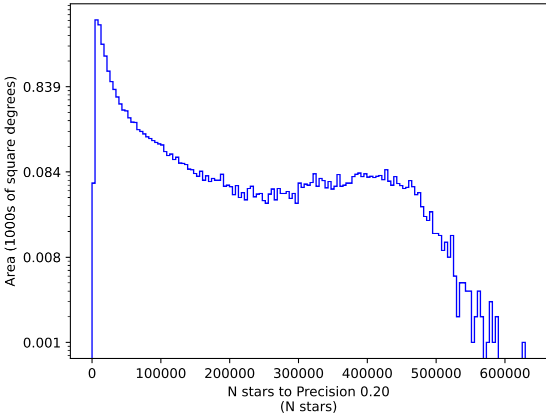
all_long_v3.4_10yrs r: N stars to Precision 0.20
