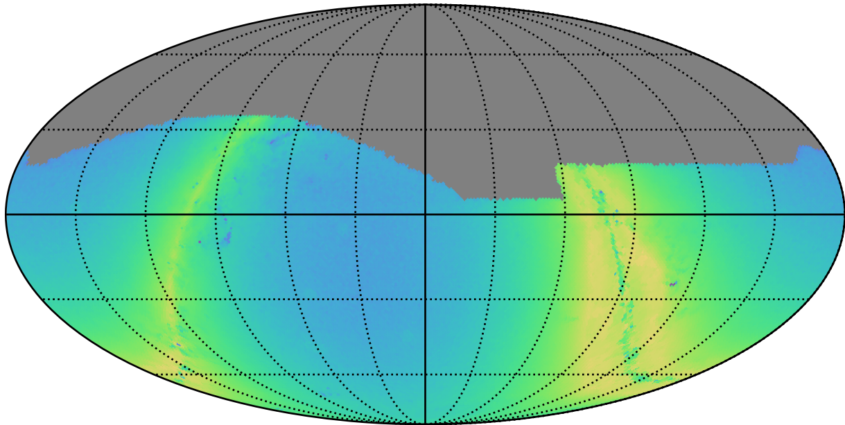
all_long_v3.4_10yrs g: N stars to Precision 0.20
