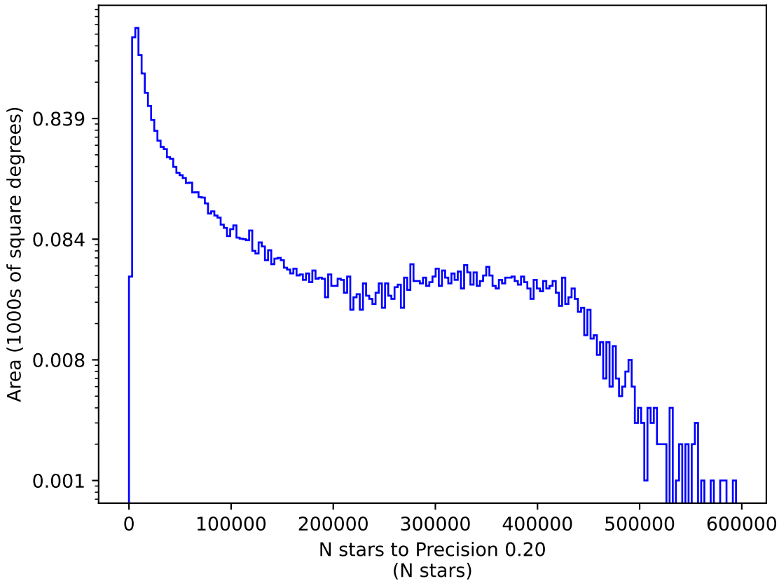
all_long_v3.4_10yrs g: N stars to Precision 0.20
