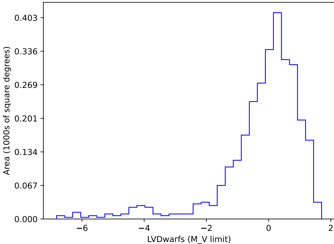
all_long_v3.4_10yrs gi SCP: LVDwarfs
